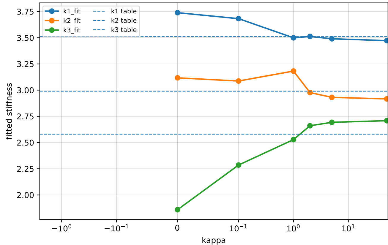
Reconstructed PRB Stiffness vs Load Ratio
